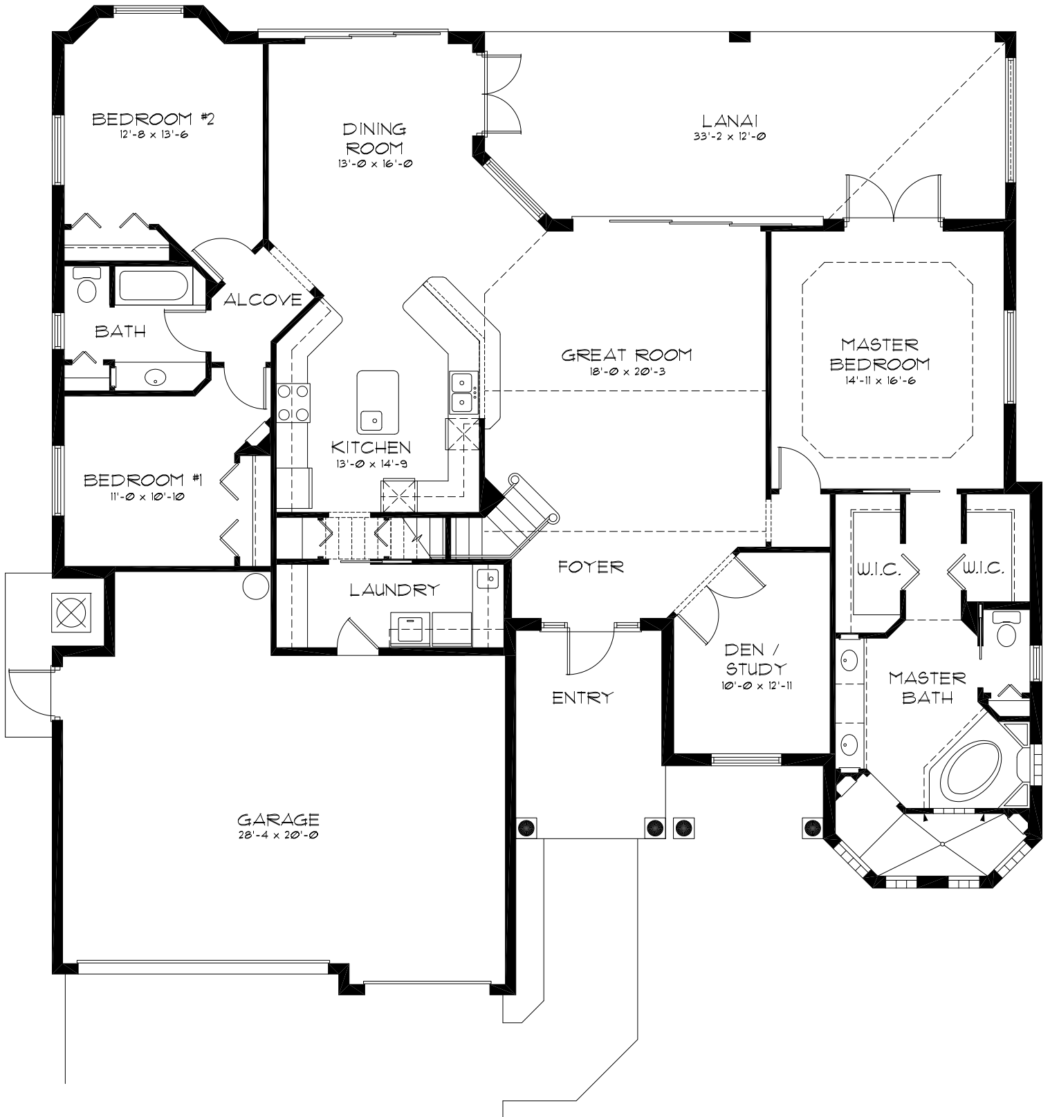
The CAPEVIEW MODEL - GROUND FLOOR
