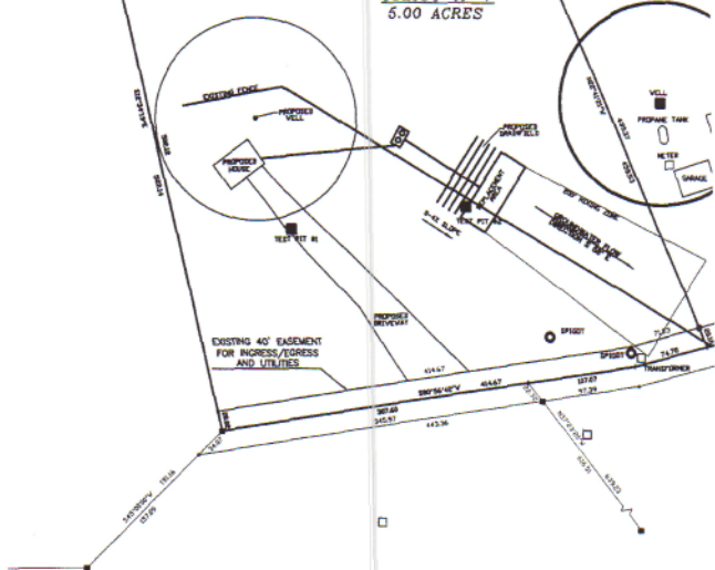
1 SITE PLAN SCALE: 1" = 100'
